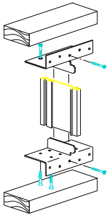
Mullion End Clip 000F (Fin mull anchor clip) Detail D
